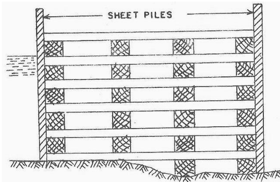
Fig: Braced Cofferdam Construction Details
