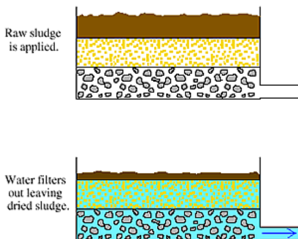
Figure-: Diagram depicting operation of a drying bed
